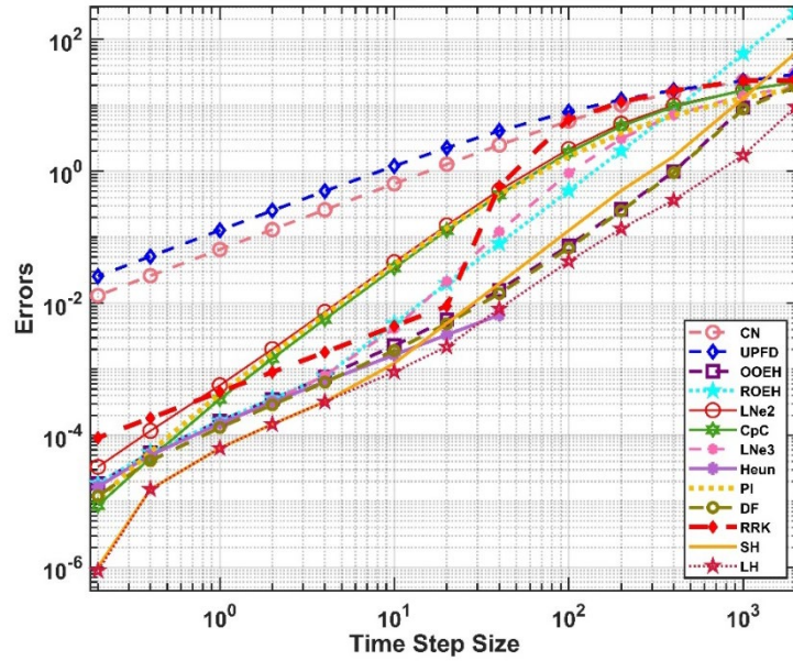
Figure 4.7. The maximum errors as a function of the time step size for the equidistant mesh for a wall with insulation.
