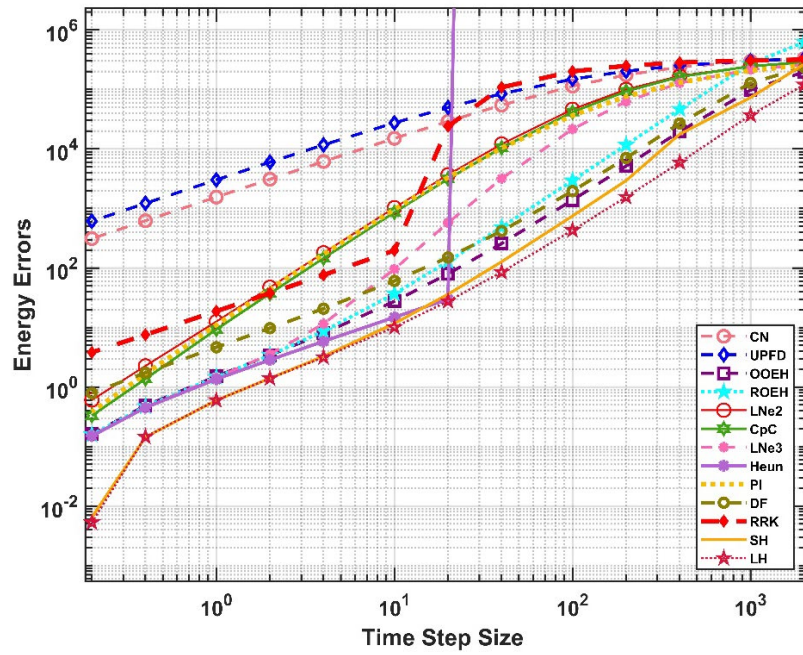
Figure 4.9. The energy errors as a function of the time step size for the non-equidistant mesh for a wall with insulation
