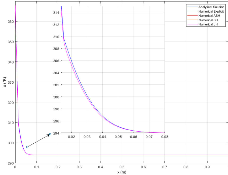
Figure 4.48. The values of temperature u along x -axis in case of the analytical solution and the numerical methods (Explicit, ASH, SH, and LH).
