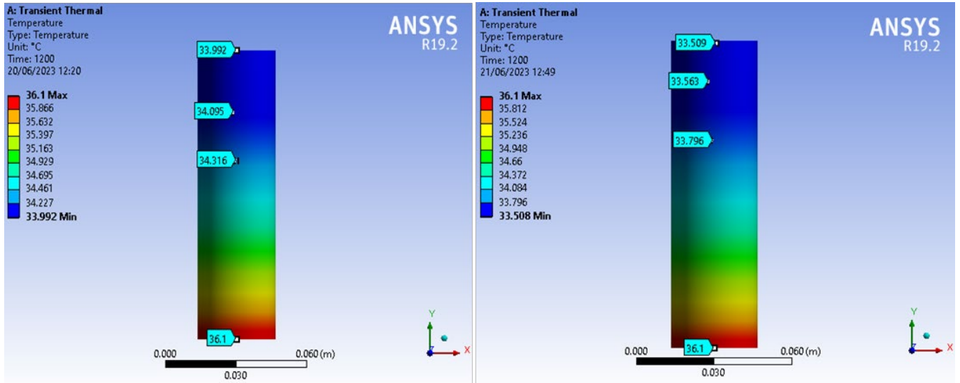
Figure 4.31. The temperature contour at time ( t = 20 min) presented by Ansys when there is no heat exchange with the environment ( left ) and when there is a heat exchange ( right )
