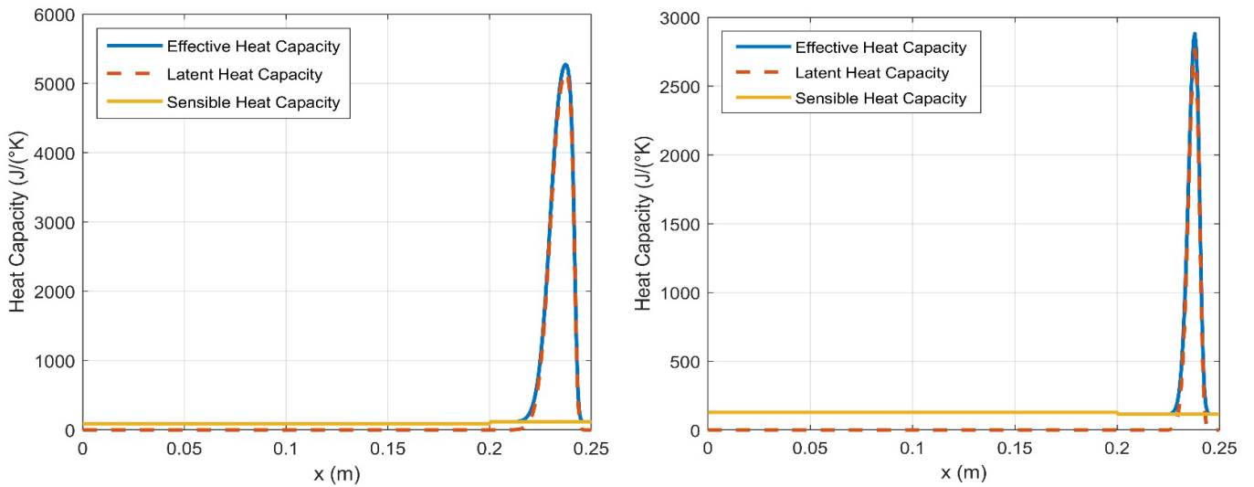
Figure 4.52. The heat capacity in Case1 for Brick+PCM1 (Left), Concrete +PCM1 (Right)
