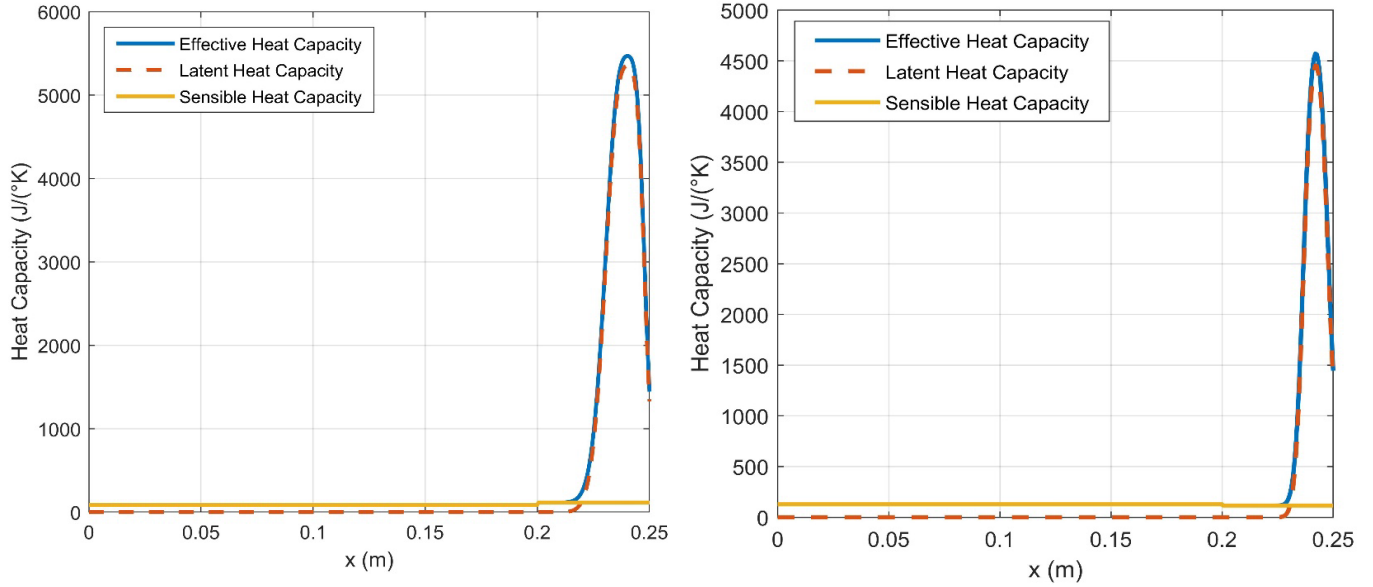
Figure 4.52. The heat capacity in Case1 for Brick+PCM1 (Left), Concrete +PCM1 (Right)
