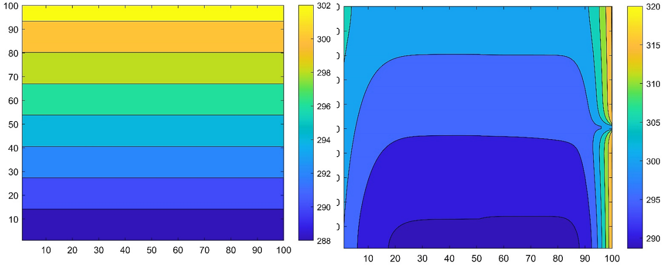
Figure 4.22. The temperature distribution contour for the equidistant mesh at initial (left) and final time (right) in case of multilayer cross-sectional area with thermal bridging.
