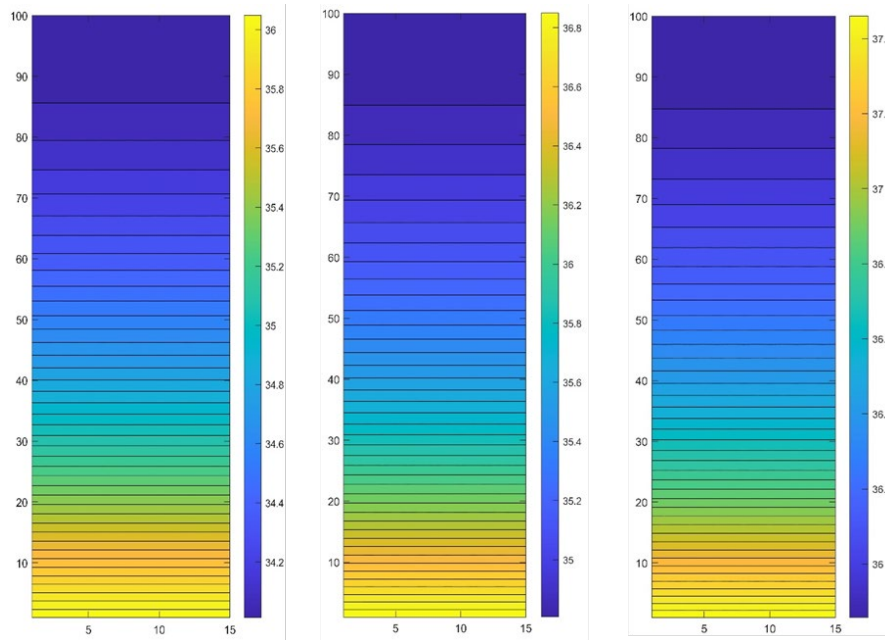
Figure 4.29. The final temperature distribution contour for different time values ( t = 20, 24 , and 30 min, respectively, from left to right) presented by the SH method when there is no heat exchange with the environment
