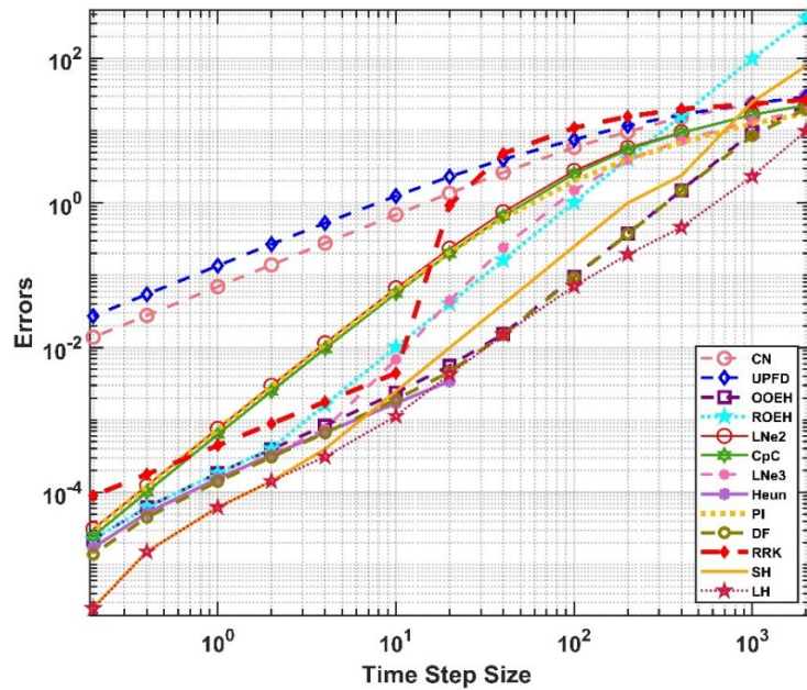
Figure 4.8. The maximum errors as a function of the time step size for the non-equidistant mesh for a wall with insulation.
