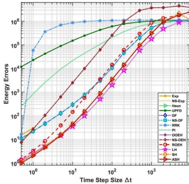
Figure 4.21. The .s as a function of the time step size for the non-equidistant mesh and thermal bridging.
