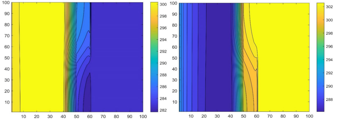
Figure 4.42. The contour of final temperature distribution in Kelvin for forced-forced convection in Case 3, in case of Cooling (left), and Heating (right).
