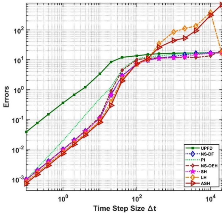
Figure 4.37. The maximum errors as a time step size function for the 7 tested methods in the case of free-forced convection cooling.
